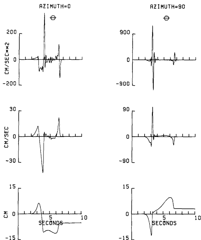
FIG. 6. Synthetic ground motion for receivers at 0^\circ and 90^\circ and epicentral range of 6 km \nu = 0.9\beta , 0.0 \text{ Hz} \leq f \leq 5.0 \text{ Hz} .
