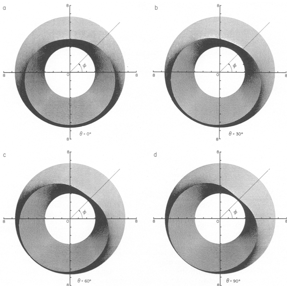
FIG. 8. The arrival time for S -wave radiation from the initiation and healing phases for successive concentric rings on the fault. Inner loops are from initiation, outer loops from healing. The direction of the rupture and healing relative to the station are evident. Receiver azimuths are indicated by \theta , v = 0.9\beta .
