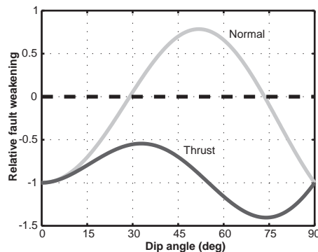
Fig. 2. The relative fault weakening (C^f - C)/\tau ahead of the crack tip at the free surface, due to fault slip at depth. \mu = 0.7 [an average value for the static friction coefficient from Byerlee's Law (24)]. A relative fault weakening of zero corresponds to the case where there is no free surface, so symmetry is not broken. With respect to the no-free-surface case, weakening >0 represents aiding the rupture, and weakening <0 represents hindering the rupture. However, any relative fault weakening >-1 corresponds to bringing the fault closer to rupture in an absolute sense.
